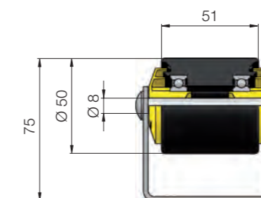
Fig.: Dimensions with polymer conveyor roller without flange
