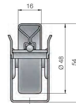
Fig.: Dimensions with steel conveyor wheels
